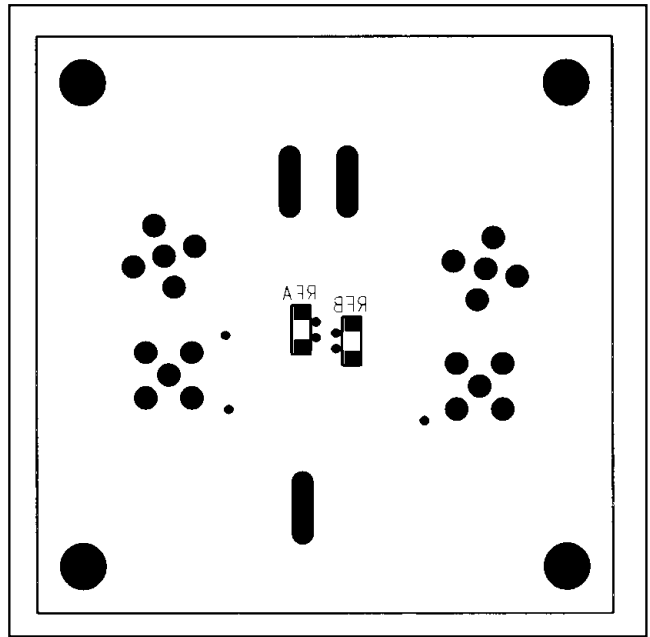
Figure 8. Component Placement Guide—Solder Side
